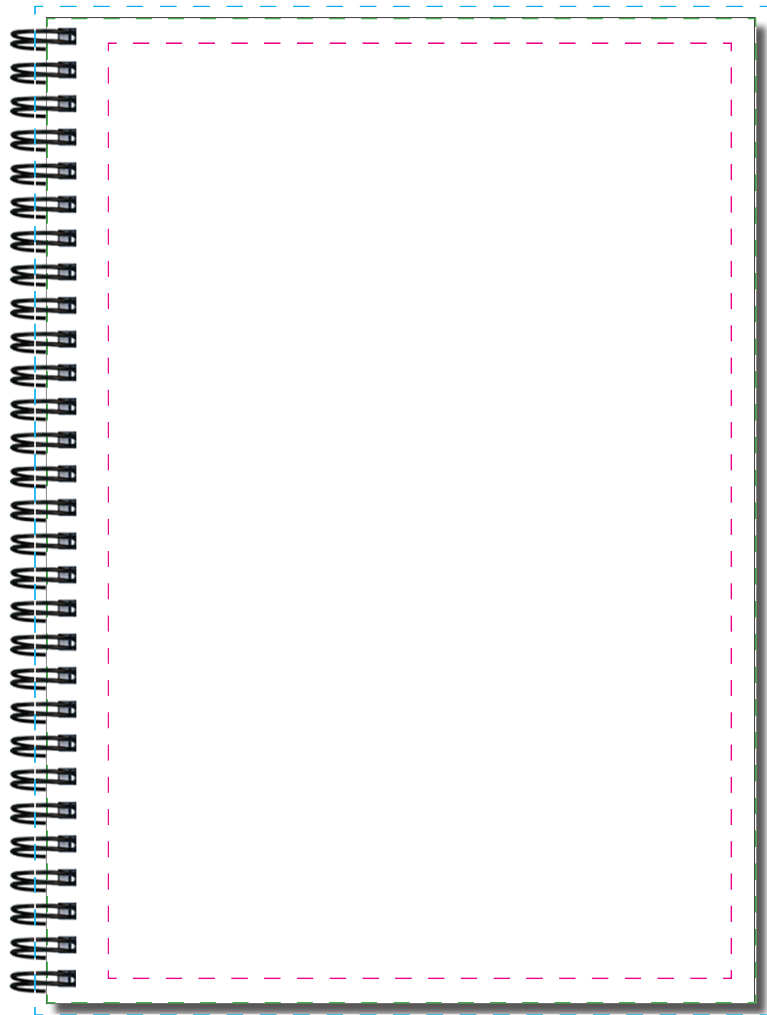
DJR - Front Cover Size: 7.25 X 10.0625 Imprint Area: 6.375 X 9.5625 Imprint Area with Bleed: 7.5 X 10.3125
